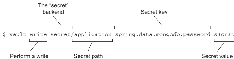
Figure 14.6 Writing a secret to Vault with the vault command
