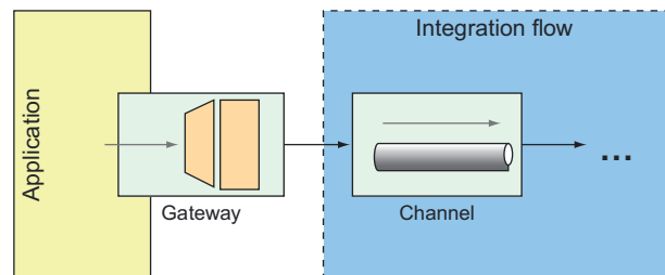
Figure 9.8 Service gateways are interfaces through which an application can submit messages to an integration flow.
